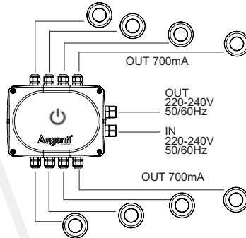
RIM45 HUB.700.001.ND MAX 8 pz. 700mA Not Dimmable
