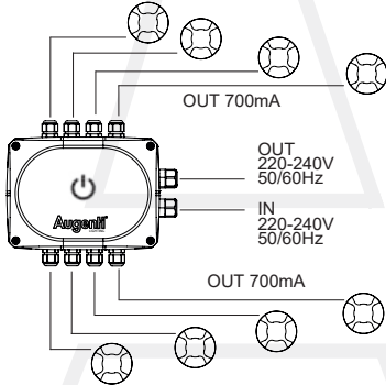
CUT45 HUB.700.001.ND MAX 8 pz. 700mA Not Dimmable
